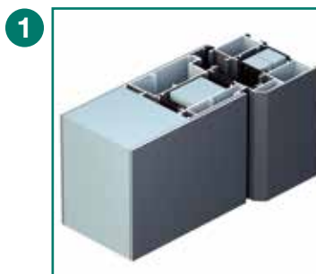
Aluminium profiles with heat barrier and additional insulation
